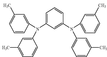
PDA
