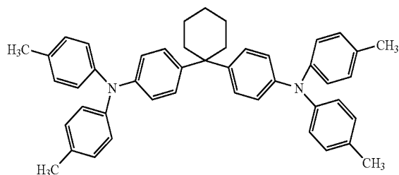
PDA
