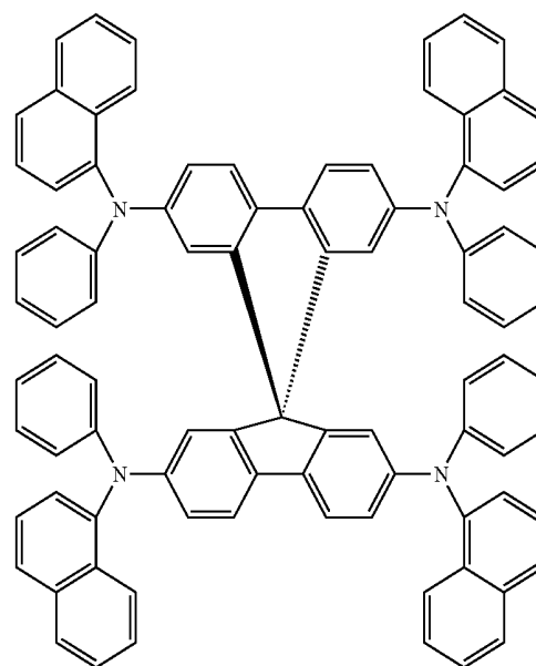
spiro-NPD
