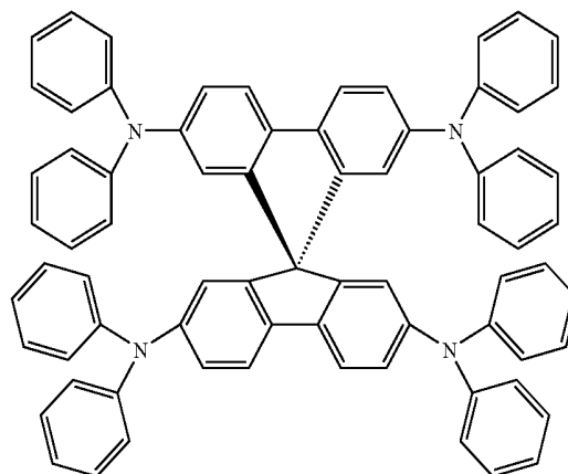
spiro-TPD
